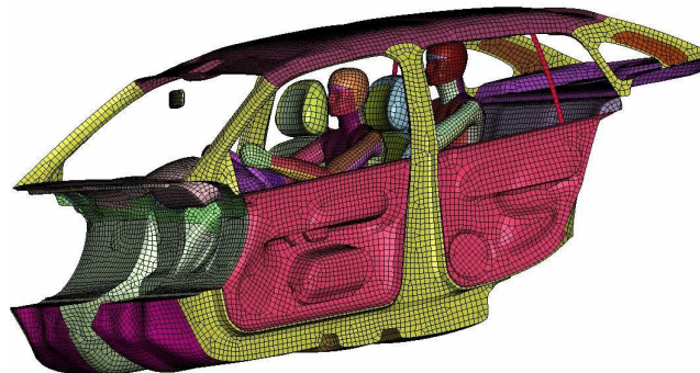
Figure 1. Section through the thermal finite element model of the vehicle with manikin inside
